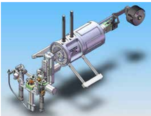
INSIDE DIAMETER PIPE WELD HEAD
